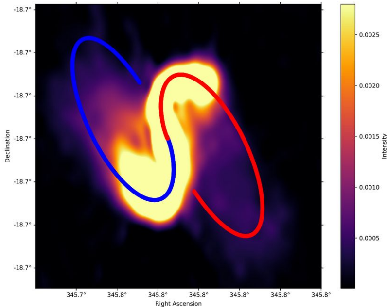
Jet precession model overlaid on VLA 6 GHz map
