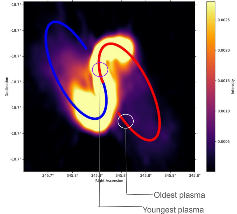
Jet precession model overlaid on VLA 6 GHz map
